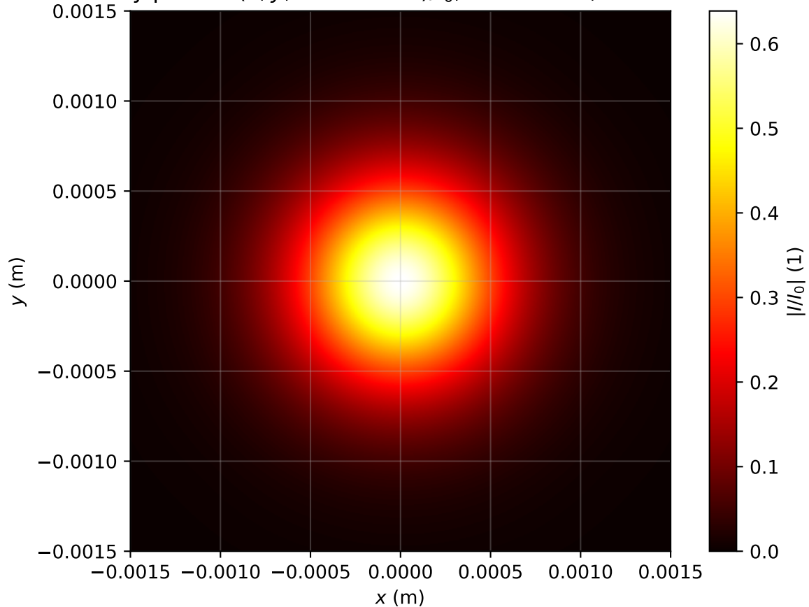
Intensity profile I(x, y, z = 3.901m)/I_0 , P_{in}=0.7P_{cr} , artificial time
